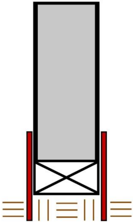
Wood Formed (Above & Below)
