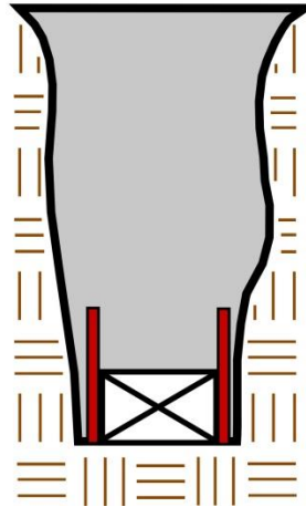
Earth Formed (Inside Trench)
